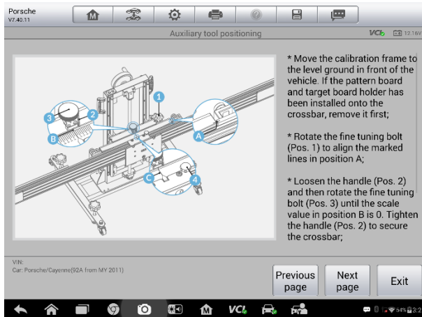
Figure 4-13 Sample Auxiliary Tool Positioning Screen
