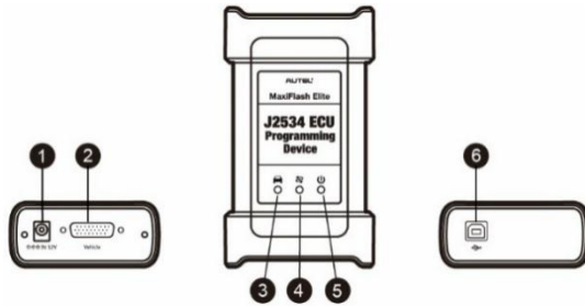
Figure 2-5 MaxiFlash Elite
